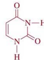
uracil (2,4-dioxypyrimidine)
