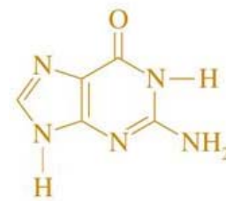
guanine (2-amino-6-oxypurine)
