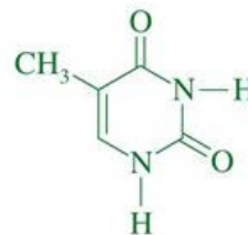
thymine (2,4-dioxy-5-methylpyrimidine)
