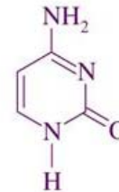
cytosine (2-oxy-4-aminopyrimidine)
