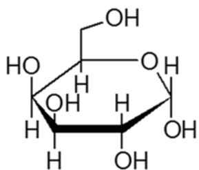
\alpha -D-Galactopyranose
