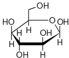
\beta -D-Idopyranose
