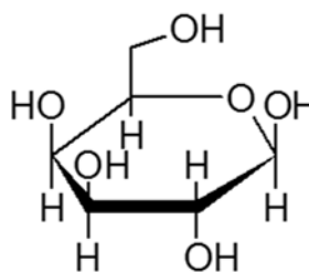
\beta -D-Galactopyranose
