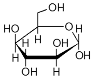
\alpha -D-Idopyranose
