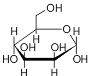
\alpha -D-Mannopyranose
