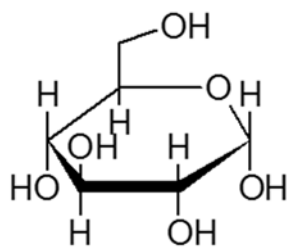
\alpha -D-Glucopyranose
