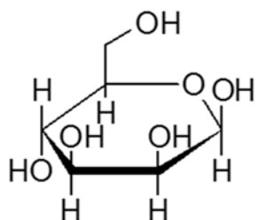
\beta -D-Mannopyranose
